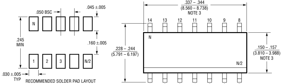
RECOMMENDED SOLDER PAD LAYOUT
